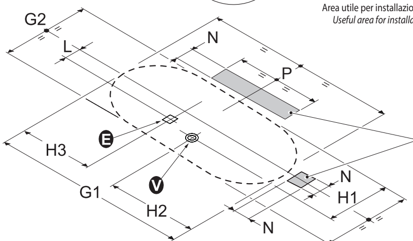
Installazione vasca in centro al locale con Rubinetteria a piantana Bathtub standing in the middle of the room with floor-mounted tapware
