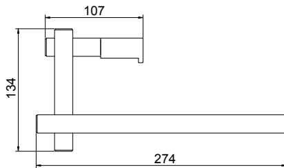
PORTA SALVIETTE SX TOWEL BAR LEFT L. 274 mm
